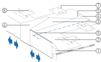
Dilatations (sliding boxes) for roof border
