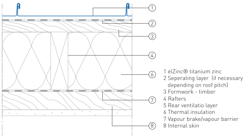
Schematic roof design of an elZinc® double lock standing seam roof with rear ventilation
