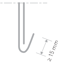
Expansion joint capping
