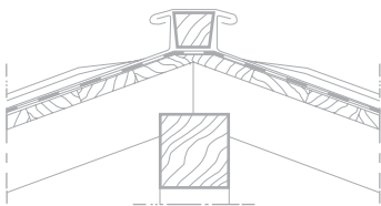
Ridge batten (in the case of transverse ventilation or separate ventilation openings between the bays)
