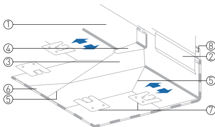
Dilatations for wall connection
