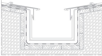
Internal gutter
