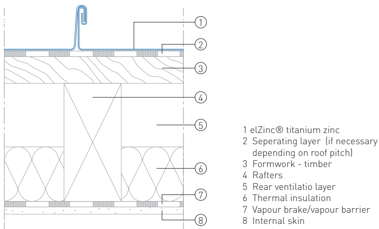
Schematic roof design of an elZinc® double lock standing seam roof with rear ventilation
