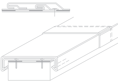
Coping with additional sliding seam
