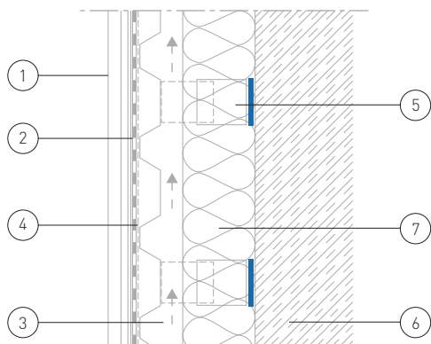
Vertical section through elZinc® titanium zinc facade with metal substructure
