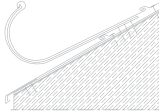
Roof-mounted gutter
